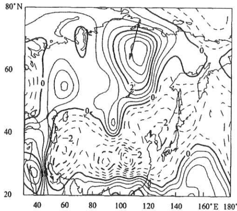
图 8 暴雨过程第 1 天 500 hPa 信号场的合成 r 值 Fig. 8. The r values of the first signal field during the process of a heavy rainfall
