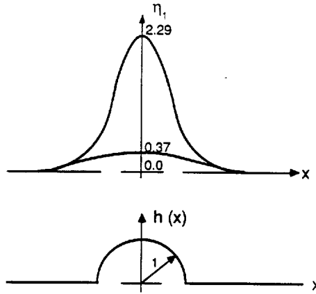
Fig. 3. Two typical supercritical solutions. F_1 = 1.4 .
