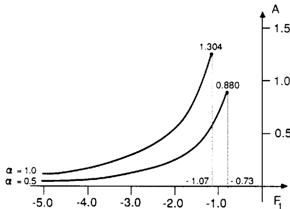
Fig. 4. Relationship between A and F_1 for subcritical solutions.
