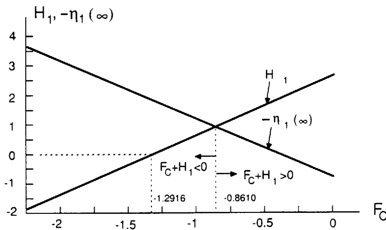
Fig. 6. H_1 and -\eta_1(\infty) vs. F_c , \alpha = 1 .
